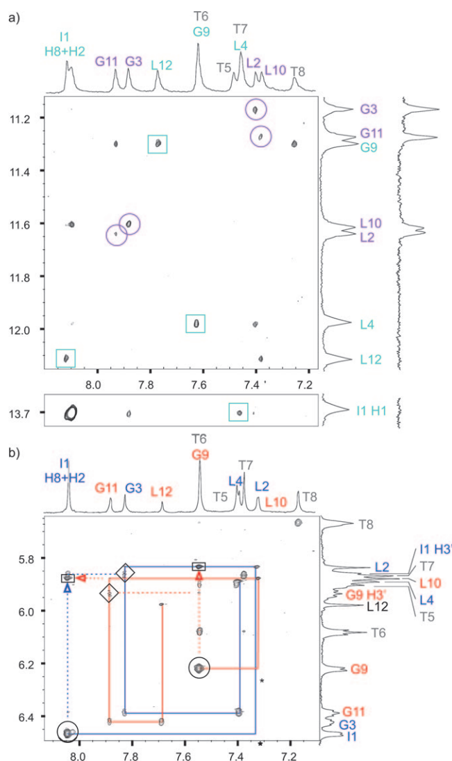
Figure 2. a) Imino to aromatic region of a 300 ms NOESY spectrum of ILGLT4GLGL in \text{H}_2\text{O} at 5^\circ\text{C} . 1D spectra with resonance assignments are shown at the corresponding axes (aromatic and imino protons horizontal and vertical, respectively). The 1D imino spectrum in \text{D}_2\text{O} after heating at 80^\circ\text{C} for 24 h is shown to the far right. Cross-peaks between G11 and G8 of neighboring bases in the tetrads are labeled with cyan squares (buried tetrads) and purple circles (exposed tetrads). b) Aromatic to \text{H}1'/\text{H}3' region of a 300 ms NOESY spectrum of ILGLT4GLGL in \text{D}_2\text{O} at 25^\circ\text{C} . 1D spectra with resonance assignments are shown at the corresponding axes (aromatic and \text{H}1'/\text{H}3' protons horizontal and vertical, respectively). The sequential connectivities between aromatic (H8) and \text{H}1' protons are indicated for I1pL2pG3pL4 (blue lines) and for G9pL10pG11pL12 (red lines). The missing sequential connectivities, I1H1'-L2H8 and G9H1'-L10H8, are marked with asterisks. Important peaks are marked with circles (I1 and G9 H8-H1'), boxes (I1H8-L10*H1' and G9H8-L2*H1'), and diamonds (I1H3'-G3H8 and G9H3'-G11H8).
